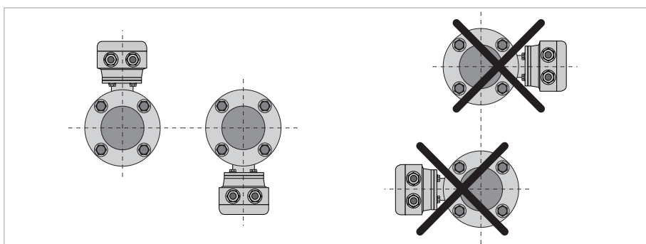
Figure 3-16: Mounting position
