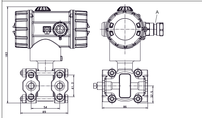
A M20 × 1.5 cable fitting
