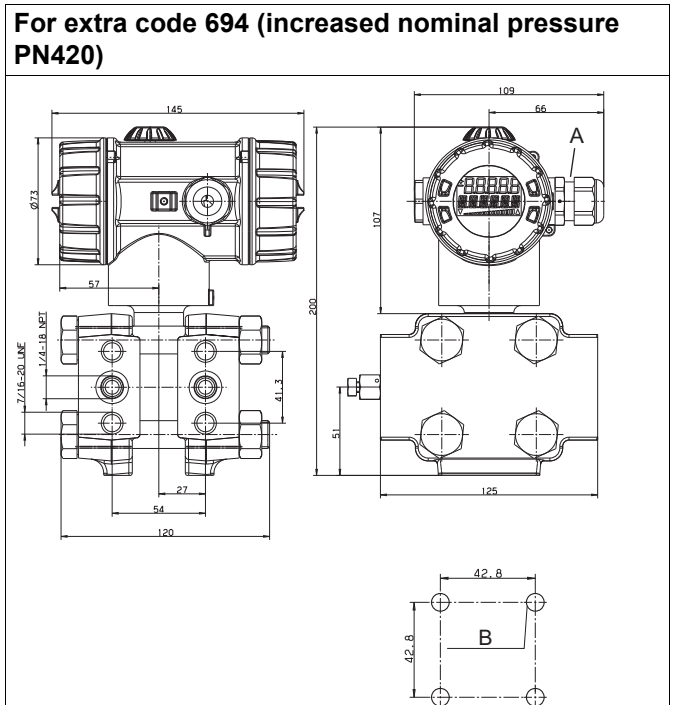
A M20 × 1.5 cable fitting B M8 for installation
